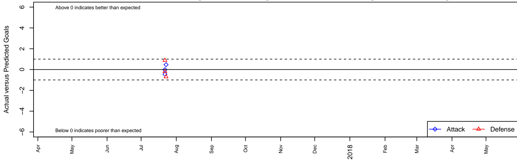
San Diego Surf Academy G05 Dots are actual minus expected GF (blue circles) and GA (red triangles). Blue line is smoothed change in attack strength. Red is smoothed change in defense strength.
